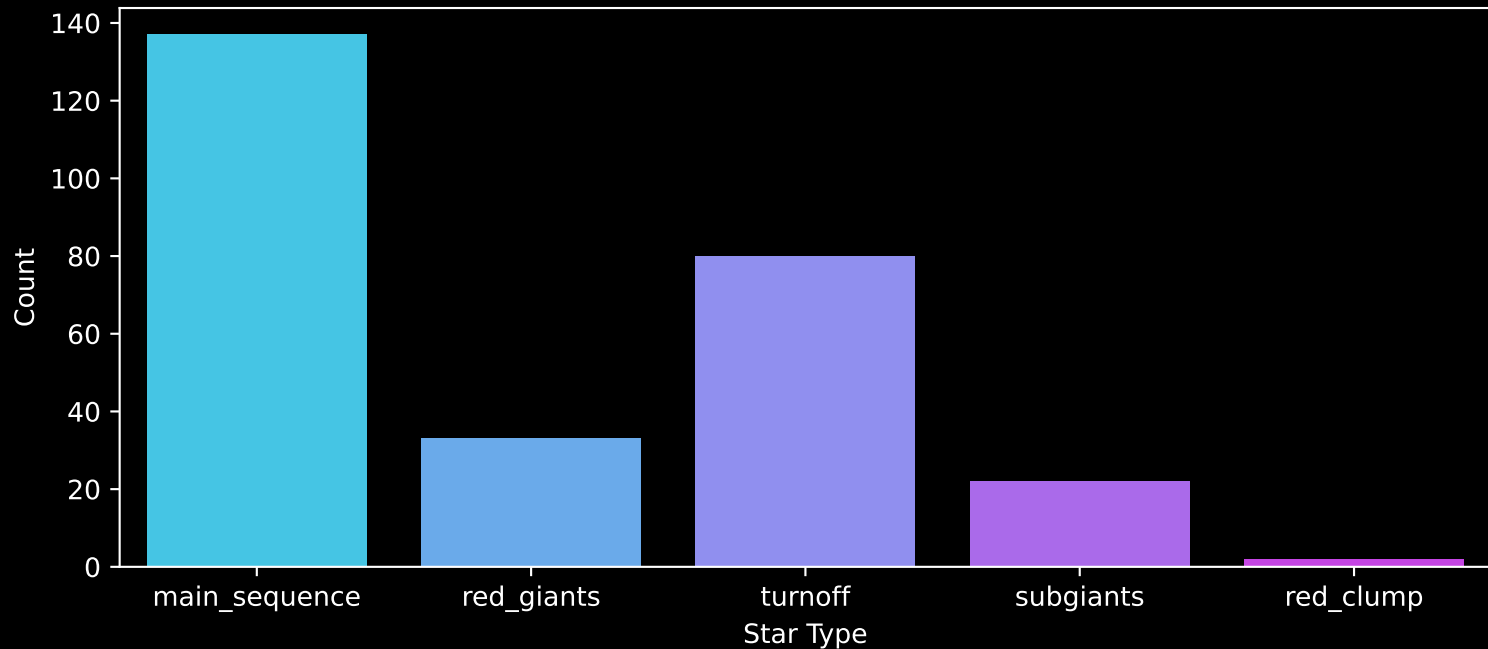
GALAH DR4 Field: [276] Count plot of Star Type
