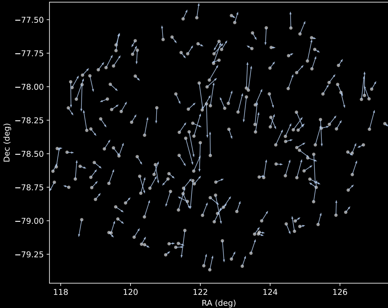
GALAH DR4 Cluster 1 Proper Motion Vectors (n=195)
