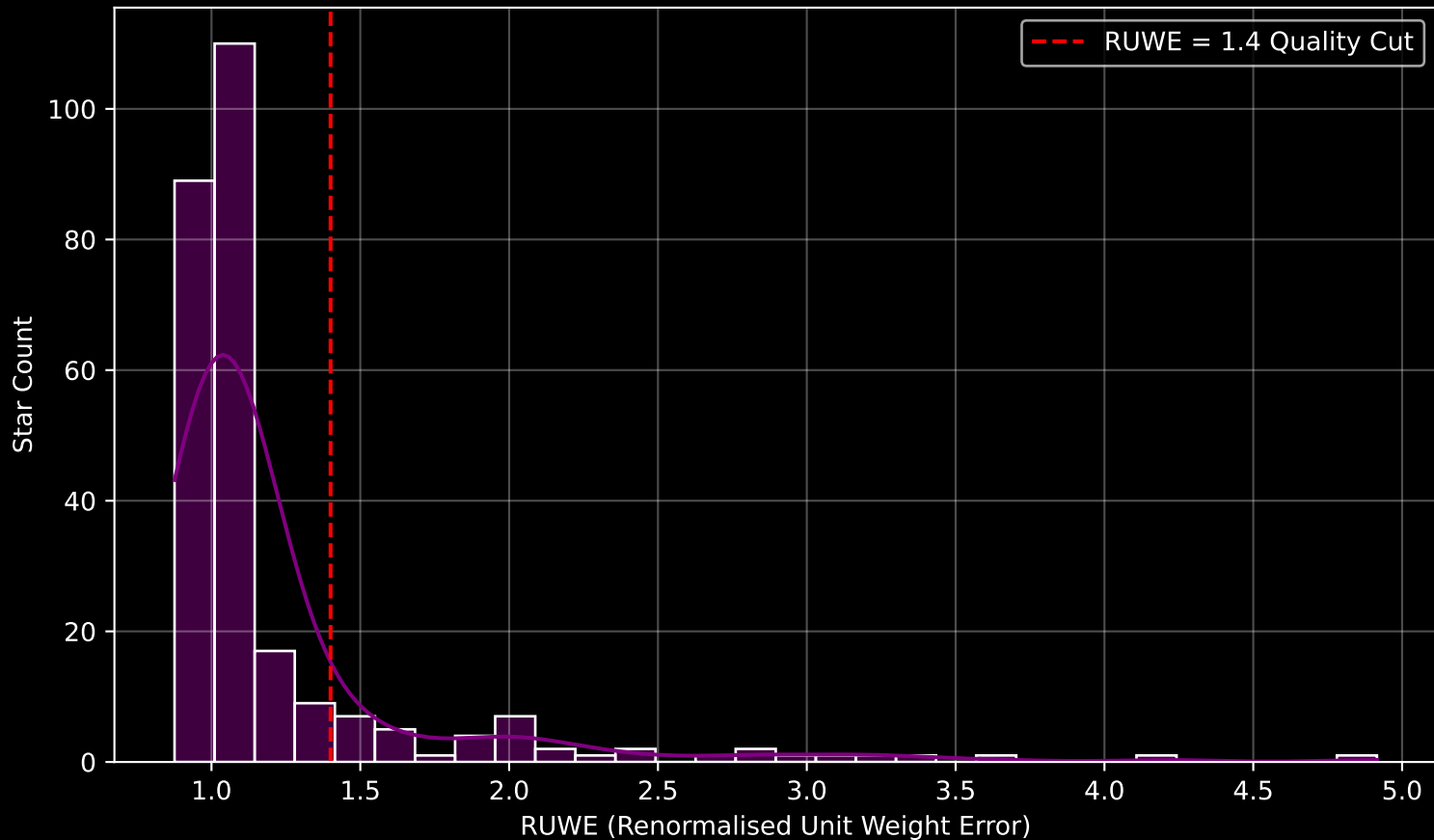
GALAH DR4 Field [276] RUWE Distribution (n= 264)
